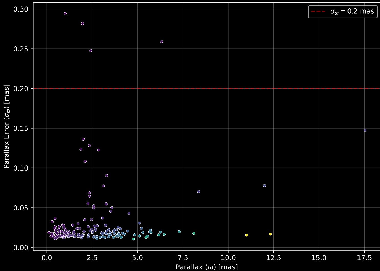
APOGEE DR17 Field: [191+26_MGA] Parallax Quality (n= 193)
