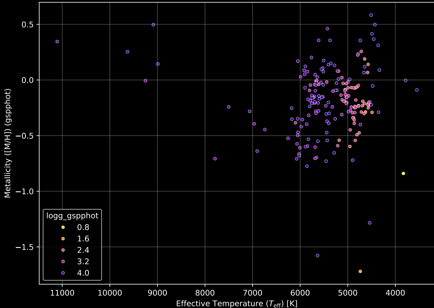
APOGEE DR17 Field: [191+26_MGA] Stellar Population Parameters (n= 193)
