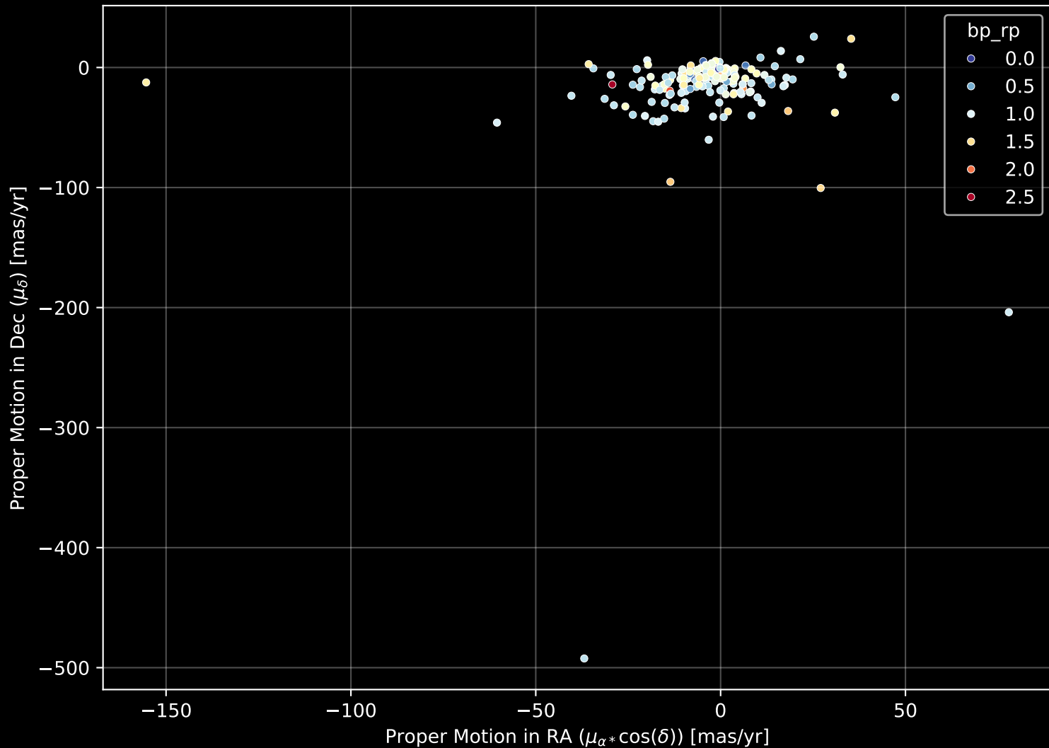
APOGEE DR17 Field: [191+26_MGA] Proper Motion Diagram (n= 193)
