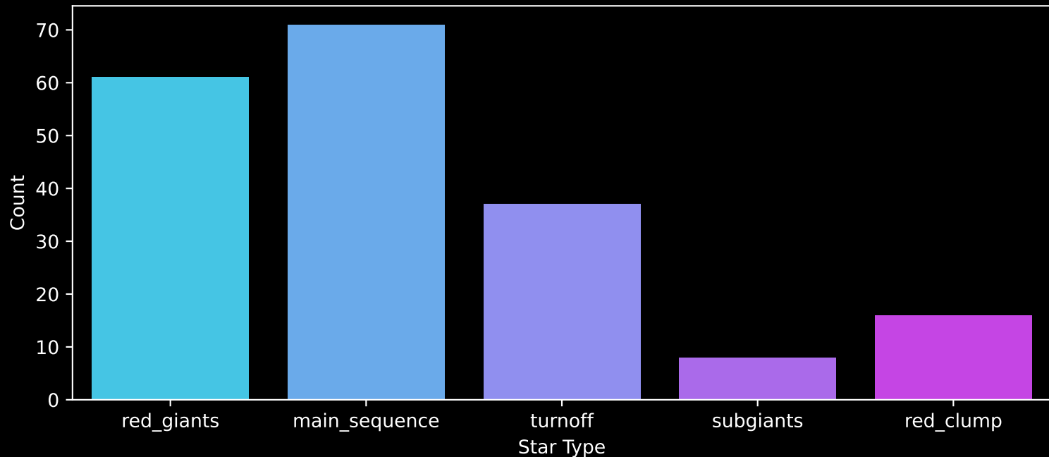
APOGEE DR17 Field: [191+26_MGA] Count plot of Star Type
