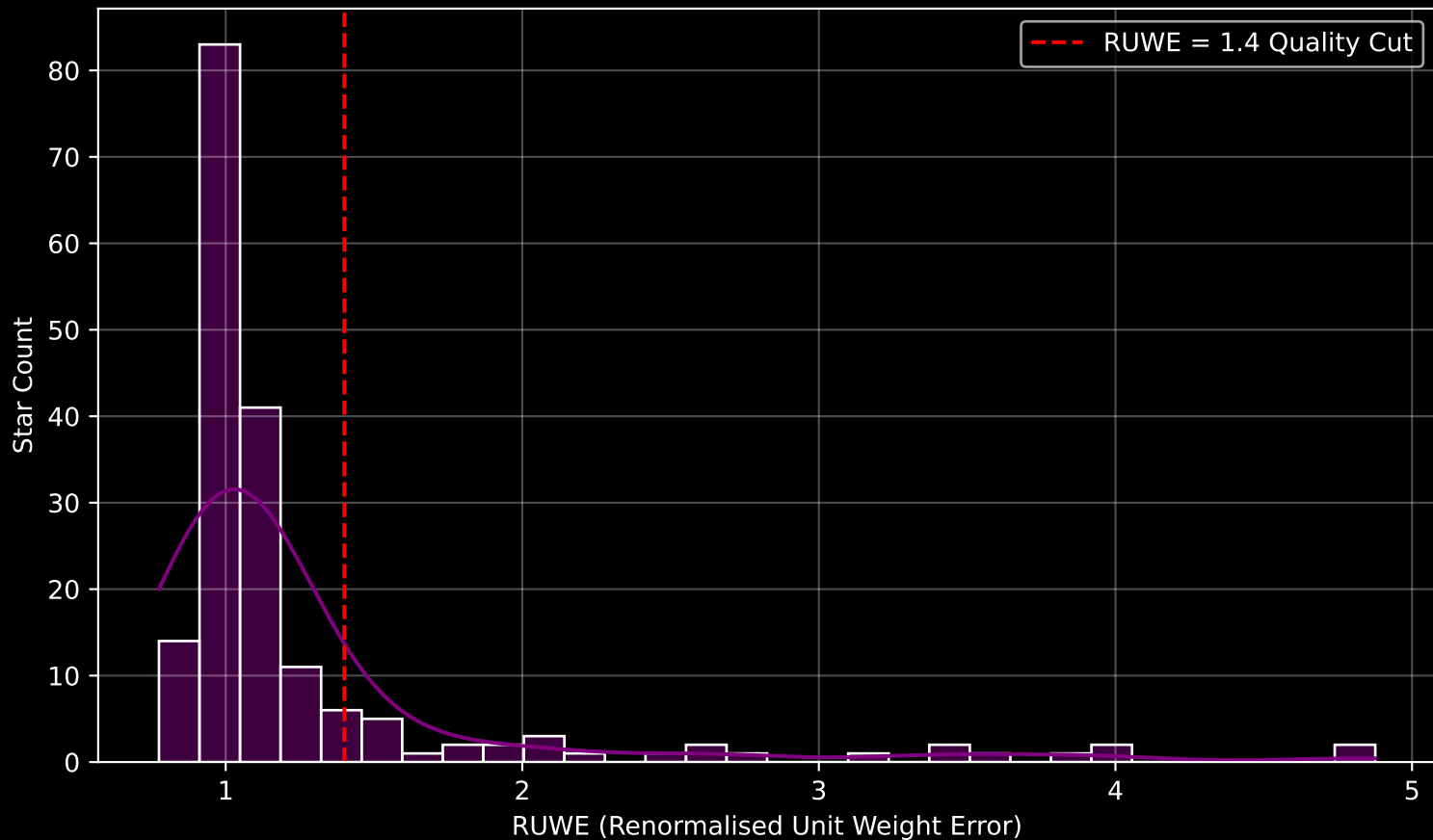
GAPOGEE DR17 Field [191+26_MGA] RUWE Distribution (n= 182)
