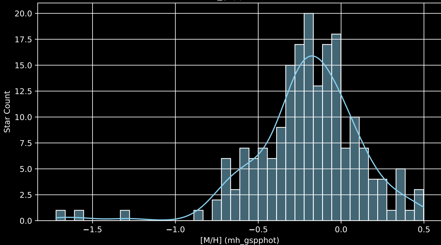
APOGEE DR17 Field: [191+26_MGA [M/H] (mh_gspphot) (n= 192)
