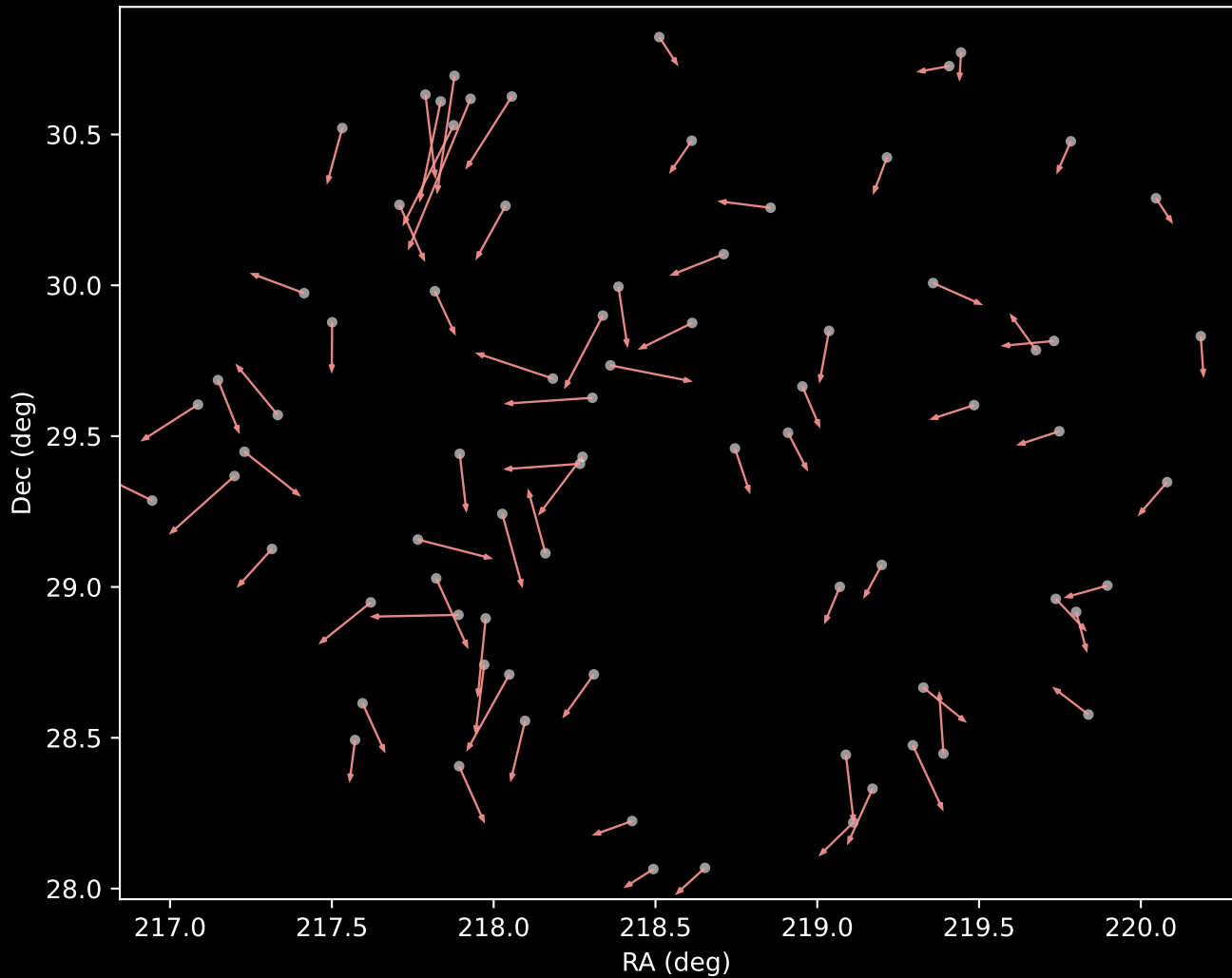
APOGEE DR17 Cluster 7 Proper Motion Vectors (n=77)
